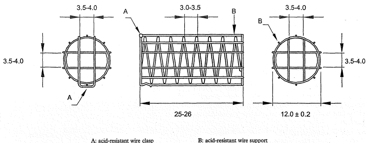
Figure 2.9.3.-3. – Alternative sinker Dimensions in millimetres
