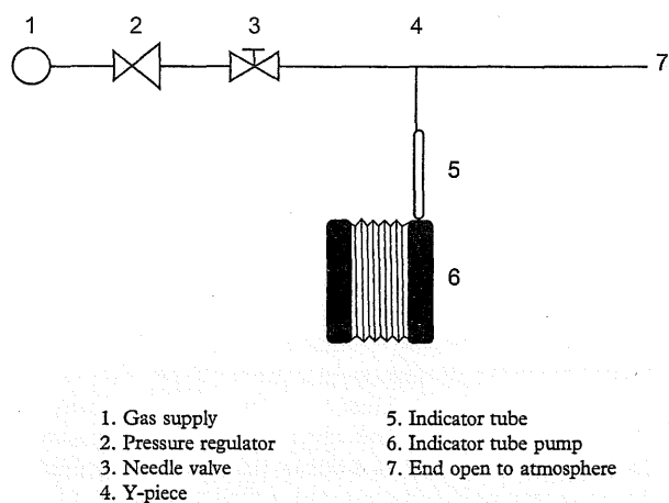
Figure 2.1.6.-1. – Apparatus for gas detector tubes
