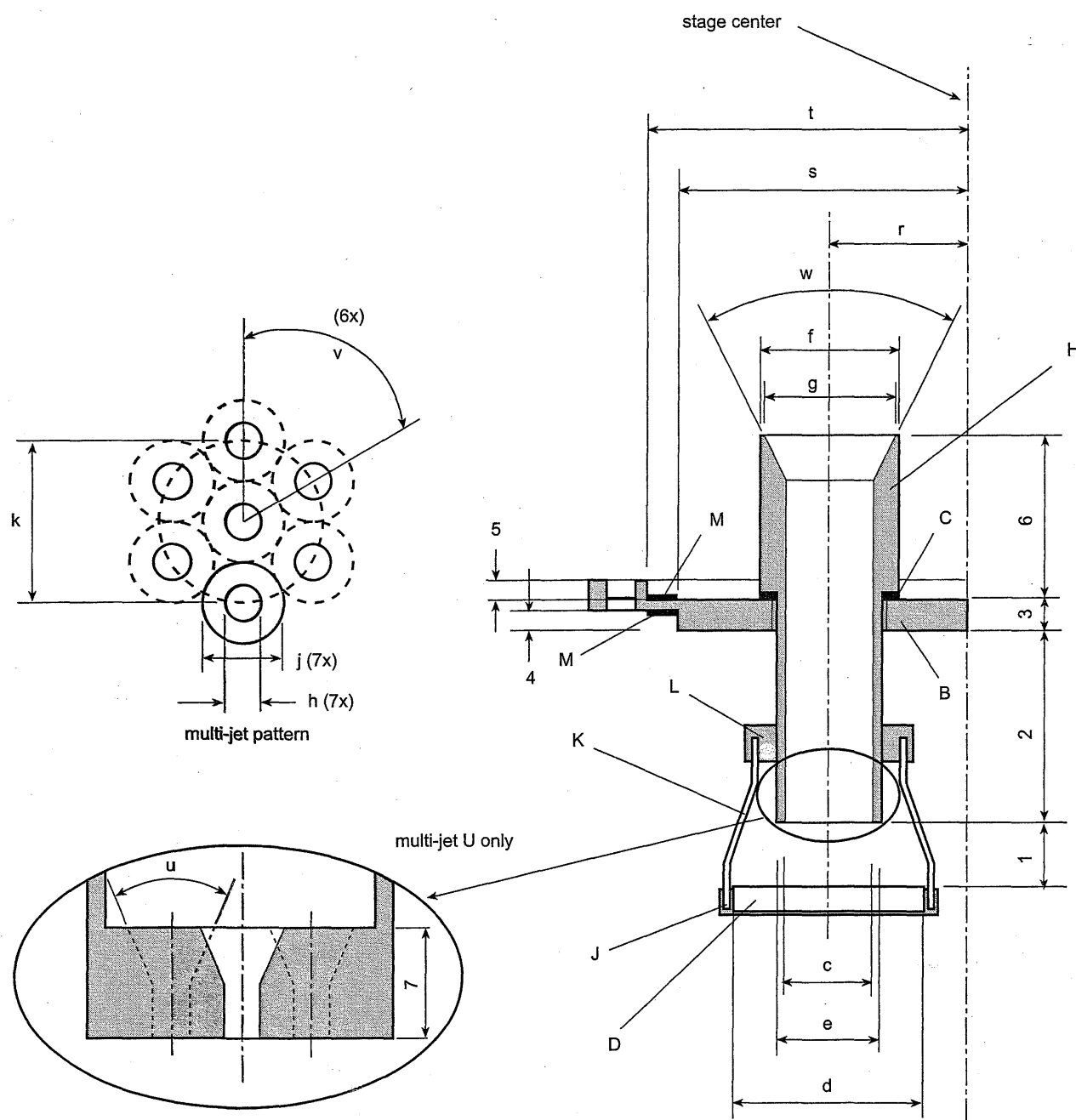
Figure 2.9.18.-5. – Apparatus C : details of jet tube and impaction plate. Inserts show end of multi-jet tube U leading to stage 4. (Numbers and lowercase letters refer to Table 2.9.18.-3 and uppercase letters refer to Figure 2.9.18.-4).
