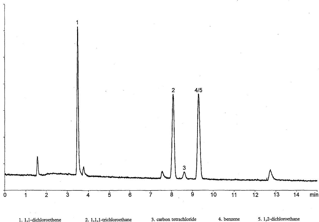
Figure 2.4.24.-1. – Typical chromatogram of Class 1 solvents using the conditions described for System A and Procedure 1. Flame-ionisation detector.
