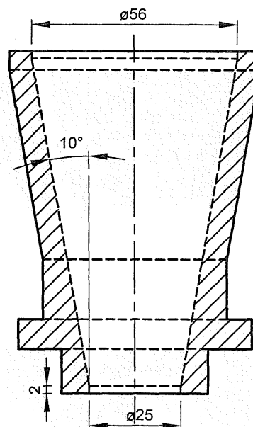
Figure 2.9.25.-2 – Funnel Dimensions in millimetres
