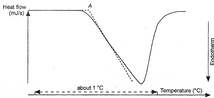
Figure 2.2.34.-1. – Thermogram
