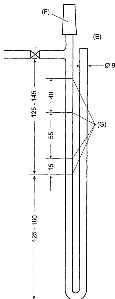
Figure 2.9.14.-2. – Manometer
