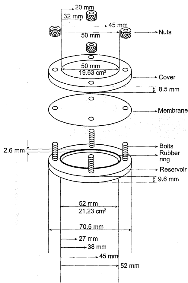
Figure 2.9.4.-3. - Extraction cell
