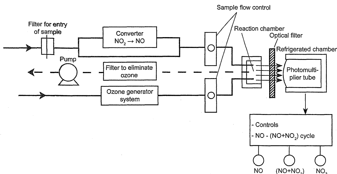
Figure 2.5.26.-1. – Chemiluminescence analyser
