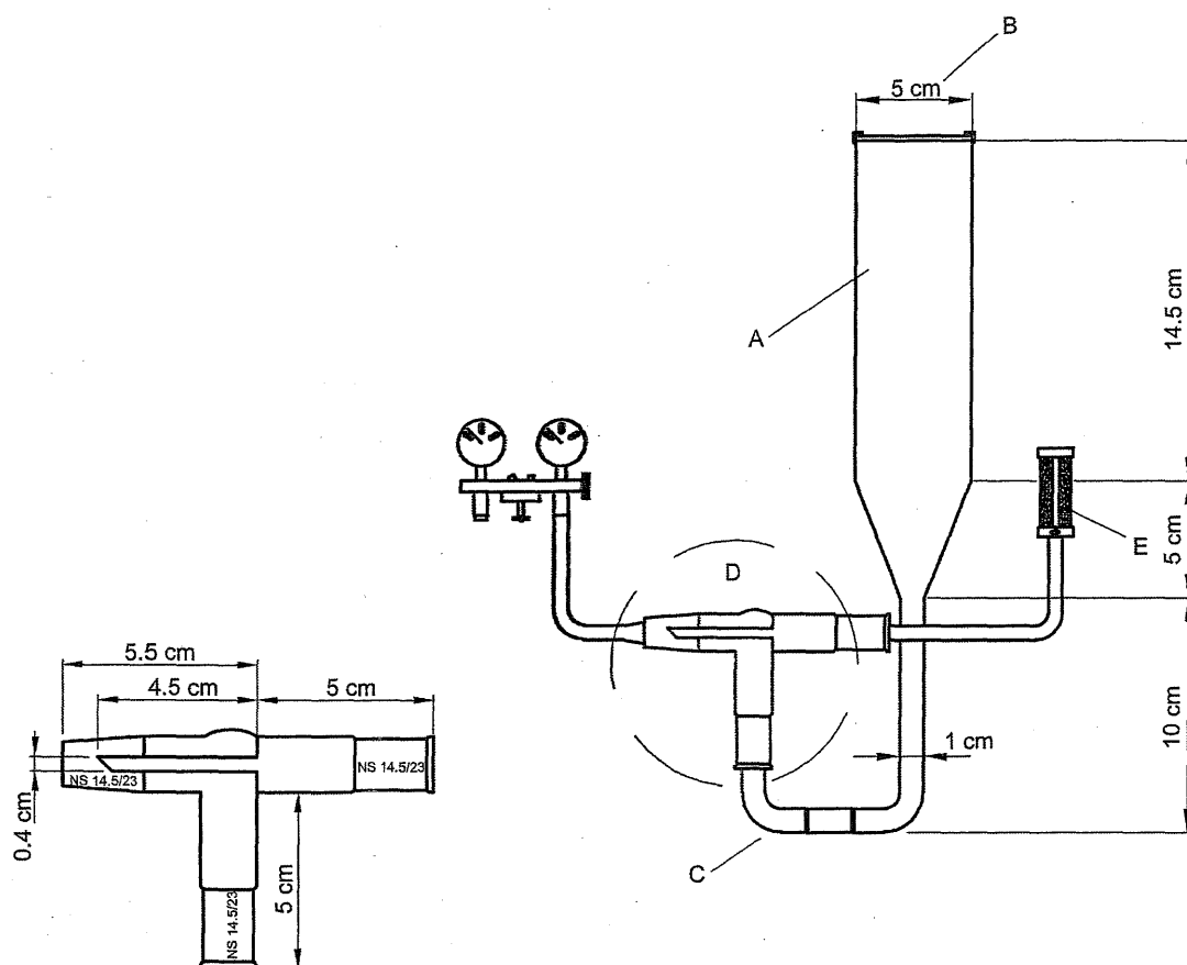
Figure 2.9.41.-1. – Fluidised-bed apparatus
