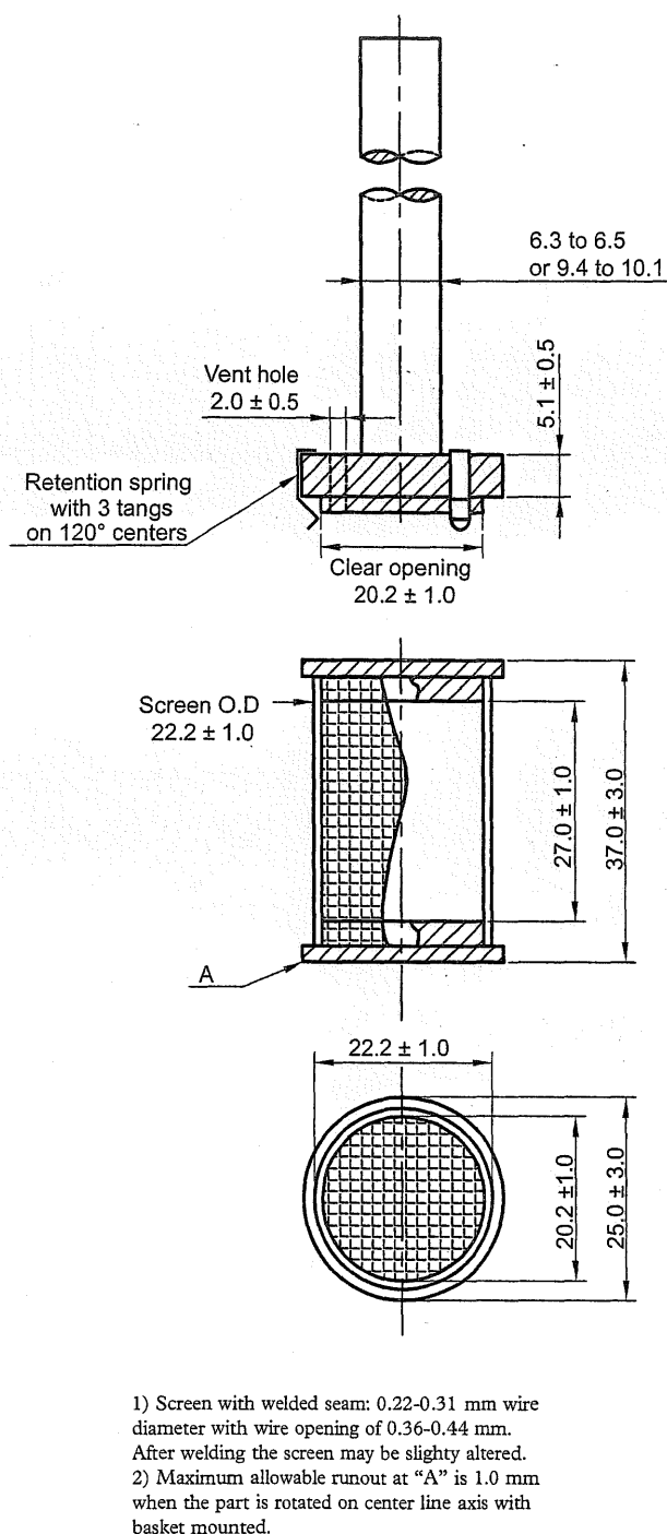
Figure 2.9.3.-1. – Apparatus 1, Basket stirring element Dimensions in millimetres
