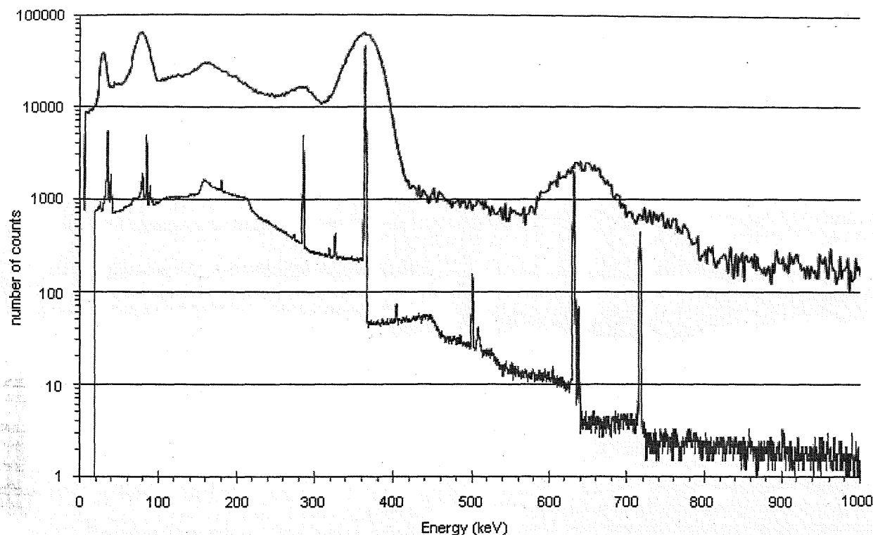
Figure 2.2.66-2. – Comparative pulse-height spectra recorded using a thallium-activated sodium iodide scintillator (upper curve) and a high-purity germanium semiconductor detector (lower curve). The source was gamma- and X-ray radiation from the decay of iodine-131.
