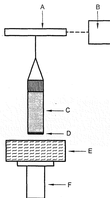
A. electronic balance C. sample holder E. immersion liquid B. computer D. filter F. lift
