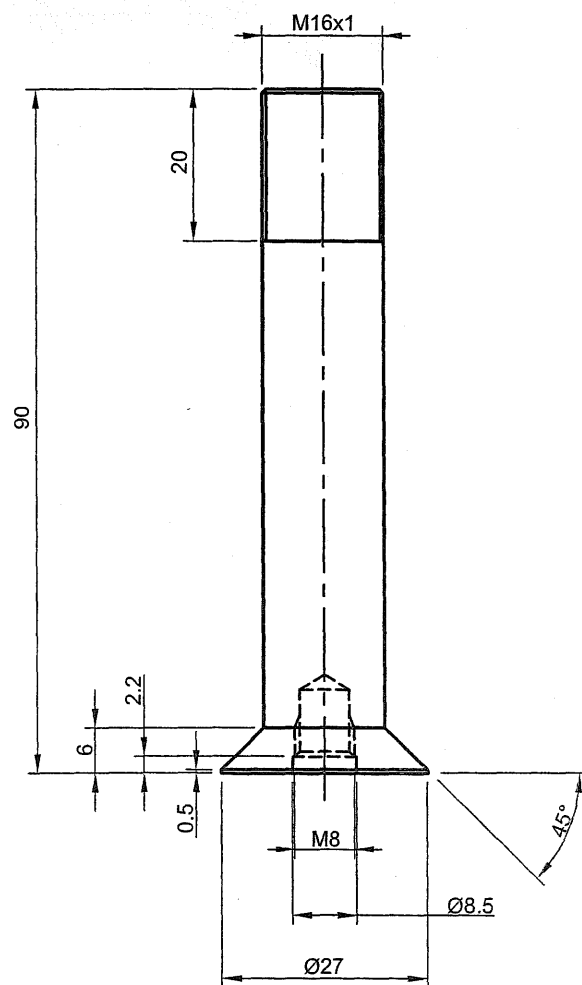
Figure 2.9.25.-7 – Axle Dimensions in millimetres
