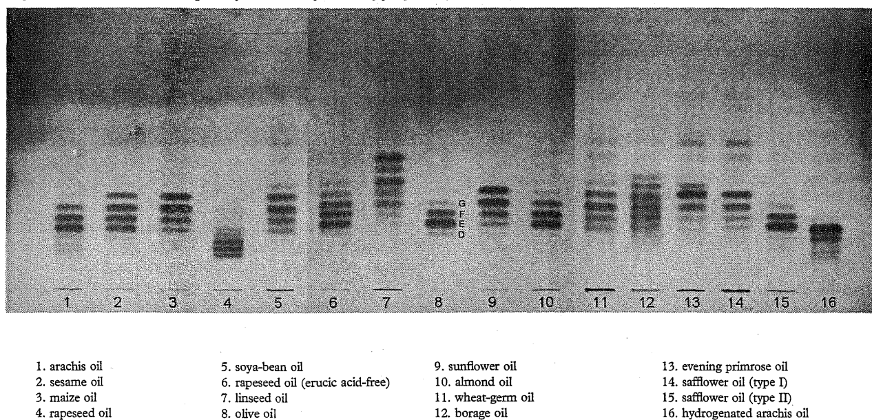
Figure 2.3.2.-1. – Chromatograms for the identification of fatty oils (method A)
