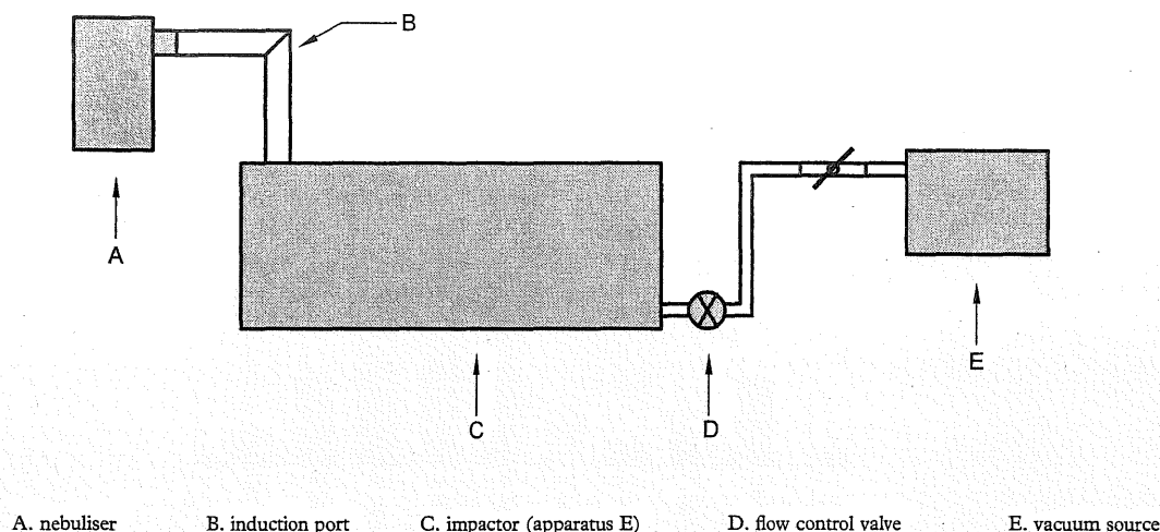
Figure 2.9.44.-2. – Apparatus E for measuring the size distribution of preparations for nebulisation
