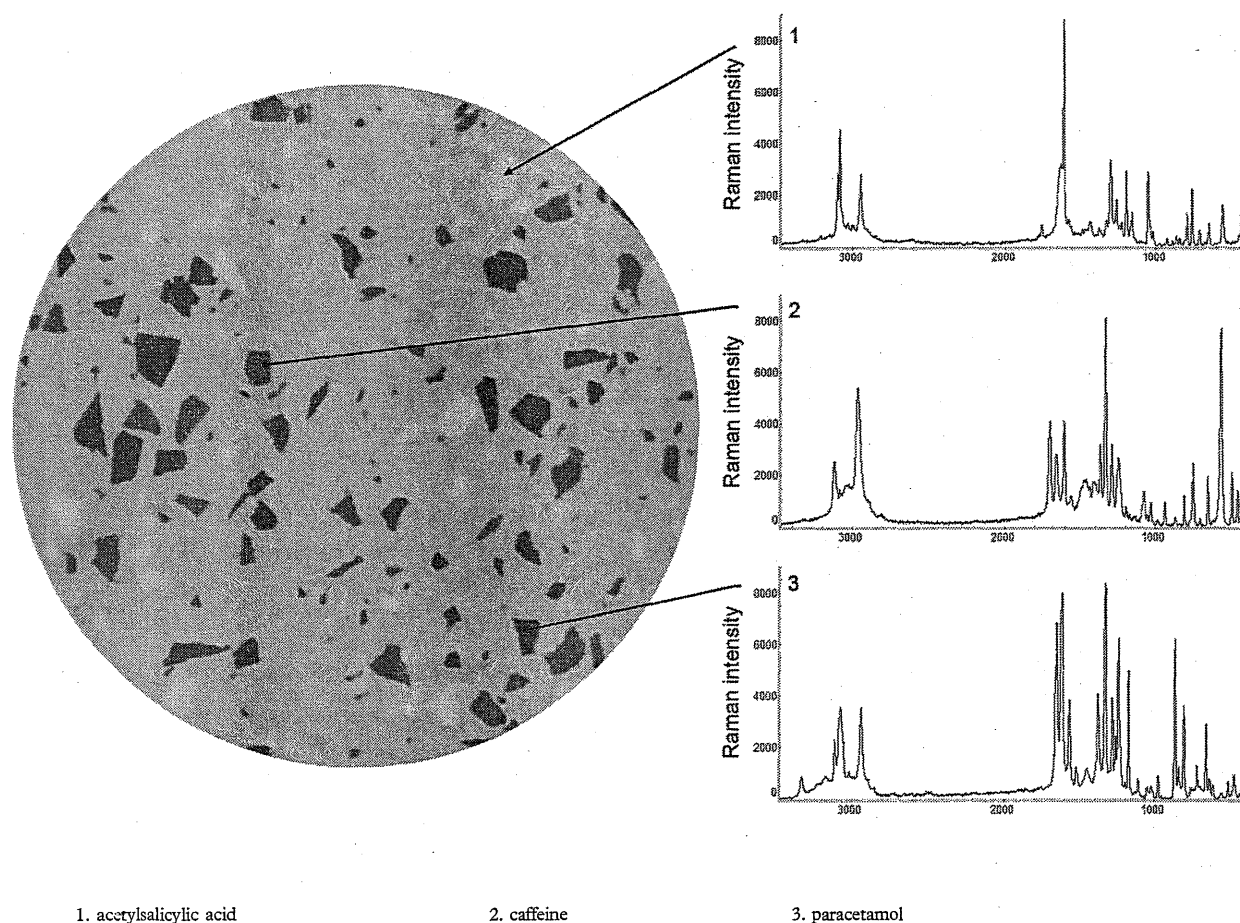
1. acetylsalicylic acid
