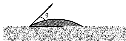
Figure 2.9.45.-2. – Sessile drop determination with visual inspection of the droplet
