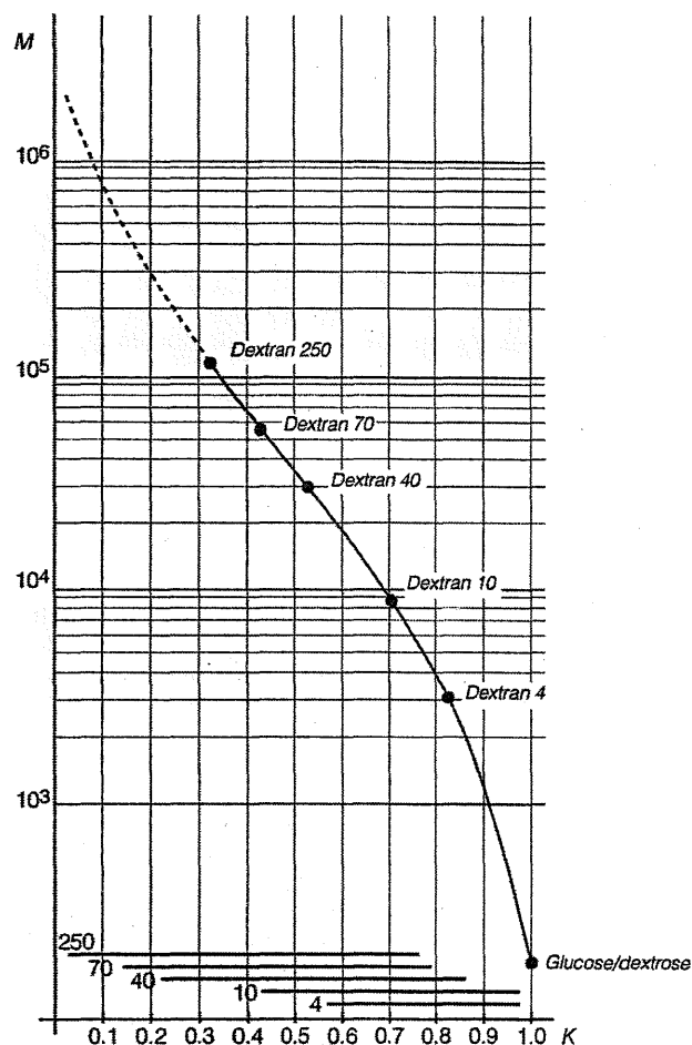
Figure 2.2.39.-1. - Example of a calibration curve.
