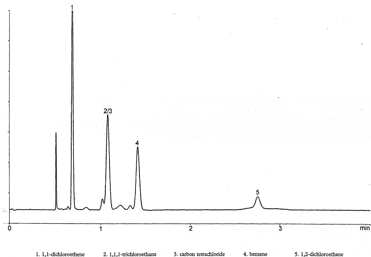
Figure 2.4.24.-3. – Chromatogram of Class 1 residual solvents using the conditions described for System B and Procedure 1. Flame-ionisation detector.
