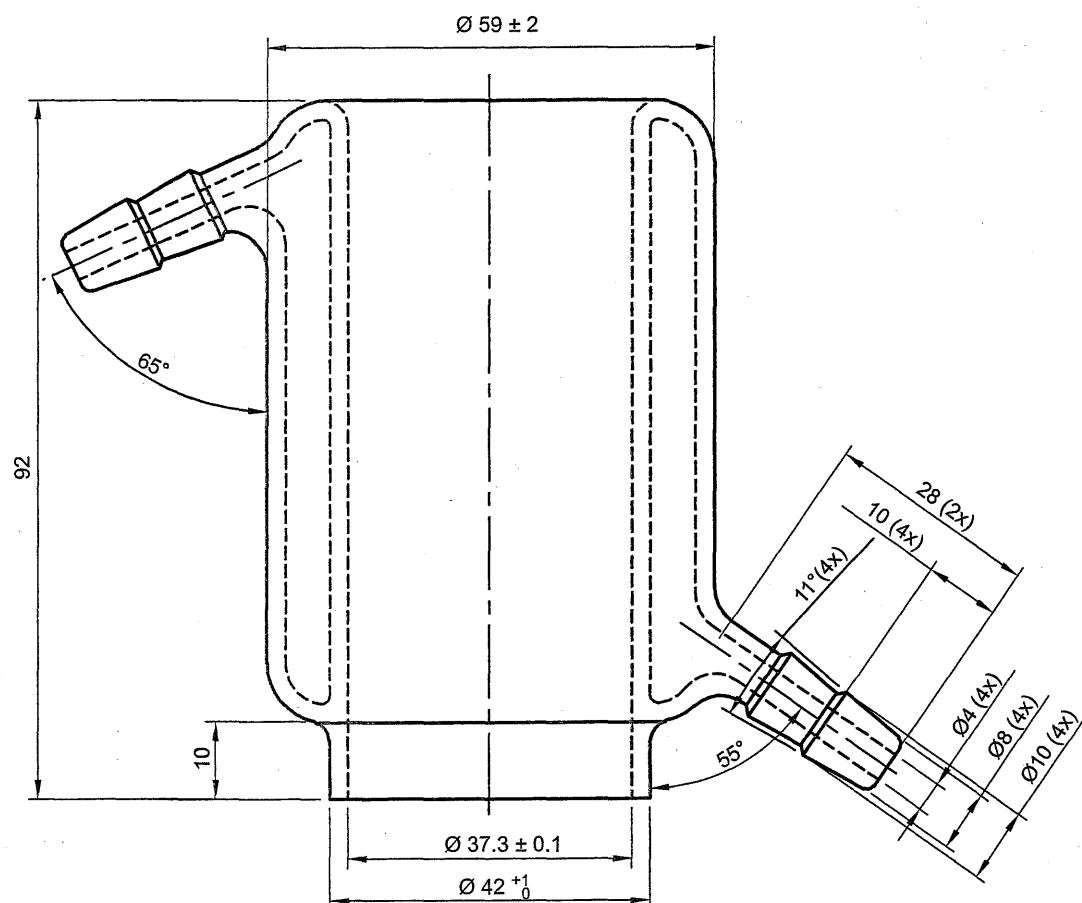
Figure 2.9.25.-5 – Test cell Dimensions in millimetres
