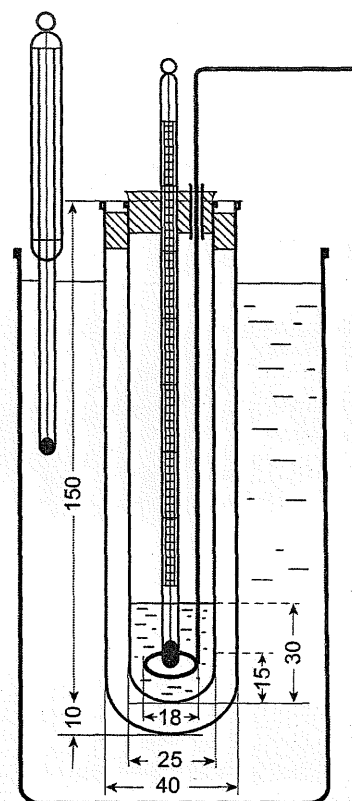
Figure 2.2.18.-1. – Apparatus for the determination of freezing point
