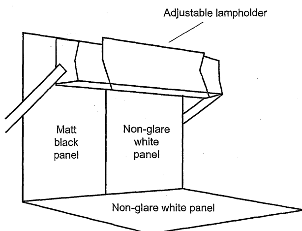
Figure 2.9.20.-1. – Apparatus for visible particles
