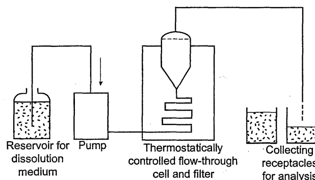
Figure 2.9.42.-1. – Flow-through apparatus
