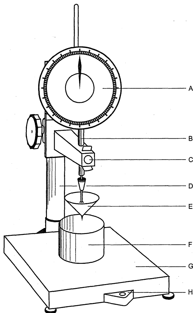
Figure 2.9.9.-1. – Penetrometer
