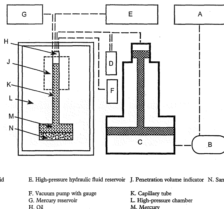
Figure 2.9.32.-1. – Example of the set-up of a mercury porosimeter instrument
