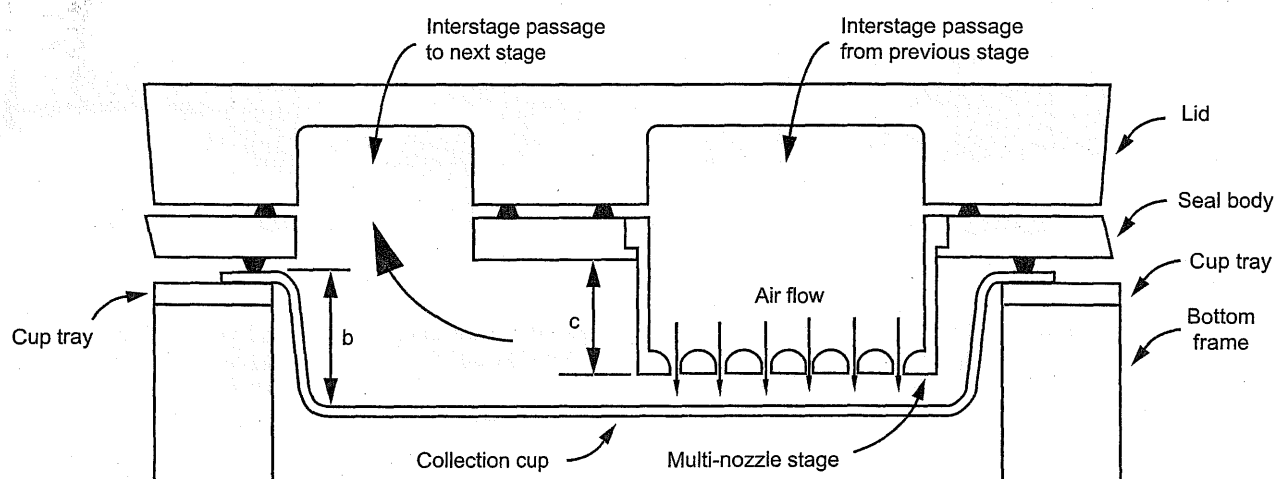
Figure 2.9.18.-14. – Apparatus E: configuration of interstage passageways
