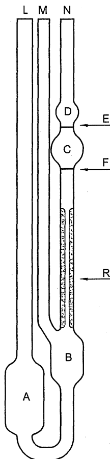
Figure 2.2.9.-1. – Suspended-level (Ubbelohde-type) capillary viscometer
