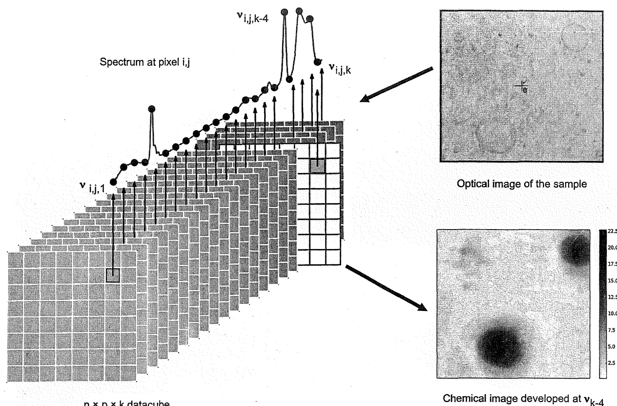
Figure 5.24.-1. – Example of a n \times p \times k datacube obtained by recording spectra of k wavenumbers at n \times p pixels of the sample; a grey-scale image was developed at wavenumber v_{k-4}
