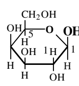
β-D-Galactopyranose
