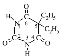
Veronal
