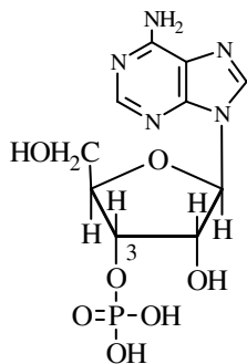
Adenylic
