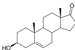
Dehydro epi androsteron
