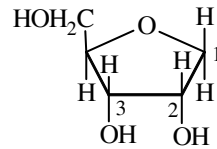
2-Deoxy-D (-)-Ribofuranose
