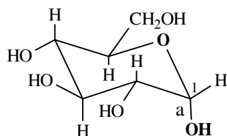
\alpha -D-Glucopyranose
