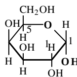
α-D-Galactopyranose
