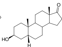
5-iso-androsteron
