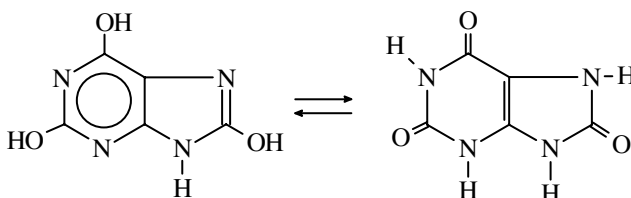
Acid Uric
