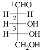
2-Deoxy-D (-)-Ribose
