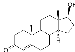
Testosteron
