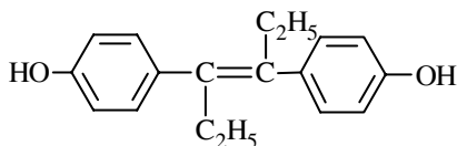
trans- Stilbestrol
