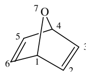
7-Oxabicyclo[2,2,1]hepta-2,5-dien
