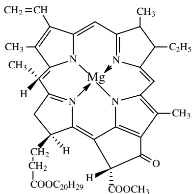
Chlorophyll a
