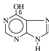
Hypoxanthin
