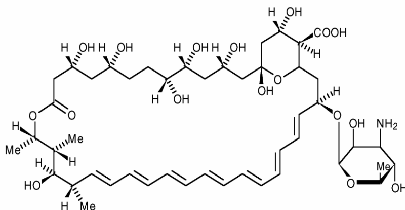
Amphotericin
