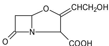
Acid clavulanic
