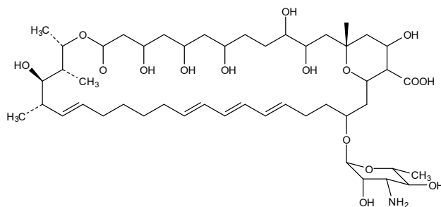
Nystatin
